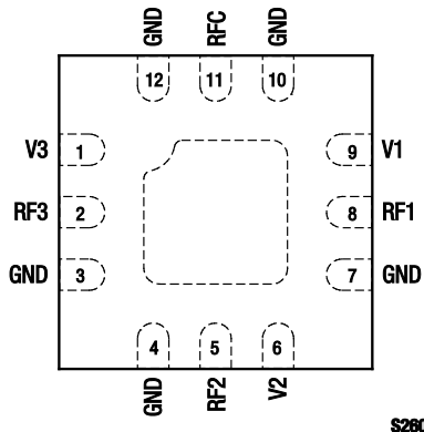
Figure 2. SKY13408-465LF Pinout – 12-Pin QFN (Top View)
