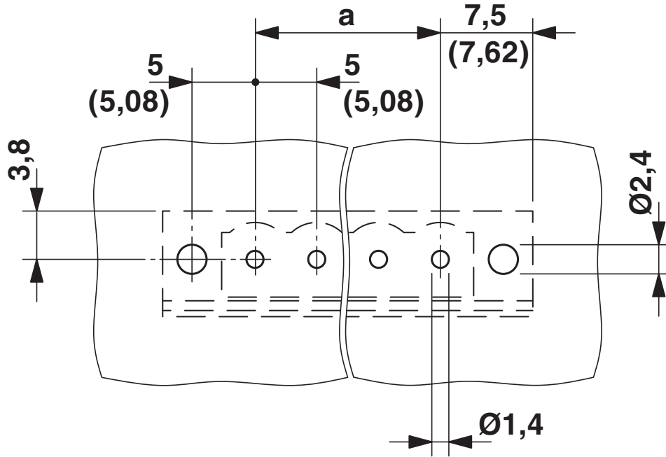
Drilling diagram
