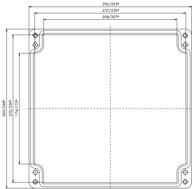
Deckel
