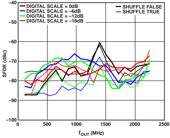
Figure 70. SFDR vs. f_{OUT} over Digital Scale
