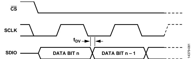
Figure 141. Timing Diagram for Serial Port Register Read
