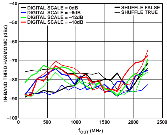
Figure 72. SFDR for In-Band Third Harmonic vs. f_{OUT} over Digital Scale
