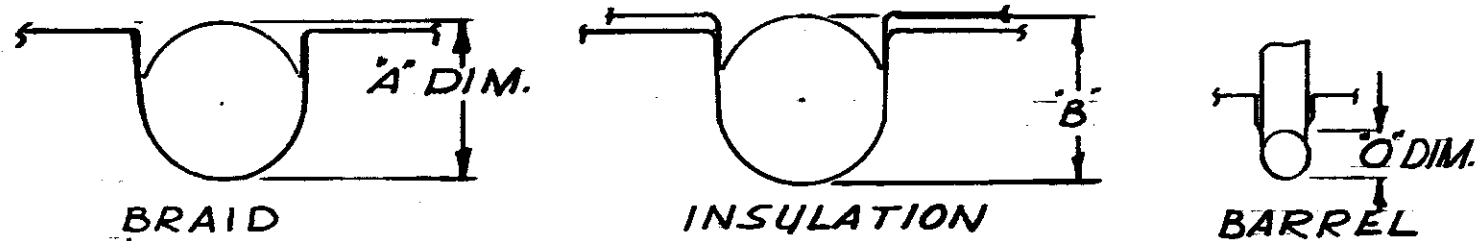
ENLARGED VIEW OF CRIMPS
