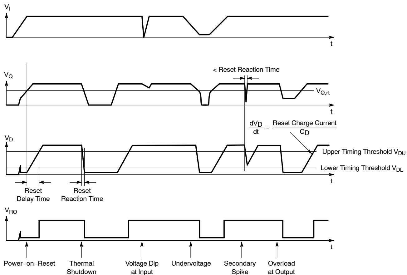
Figure 14. Reset Timing
