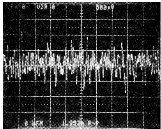
A_{\text{CL}} = 25,000\text{V/V} ; E_{\text{N}} = 0.08\mu\text{V}_{\text{P-P RTI}} Horizontal Scale = 1s/DIV; Vertical Scale = 0.02 \mu\text{V} /DIV
