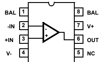
HA-5147 (CERDIP) TOP VIEW
