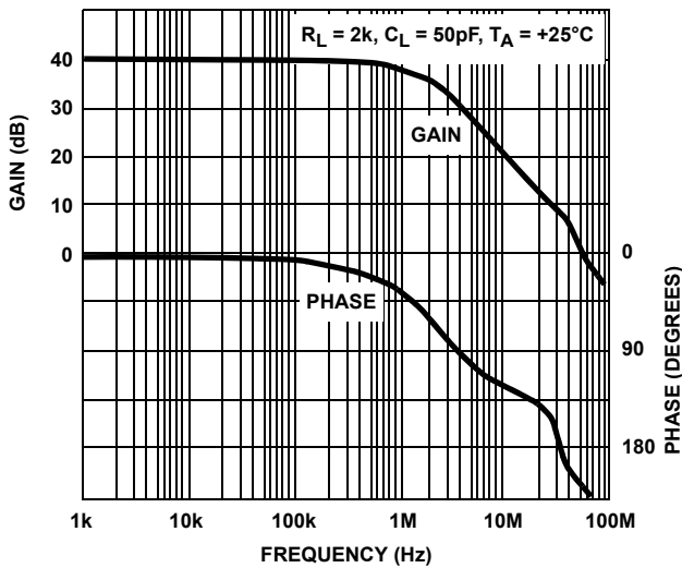
FIGURE 17. CLOSED LOOP GAIN AND PHASE vs FREQUENCY
