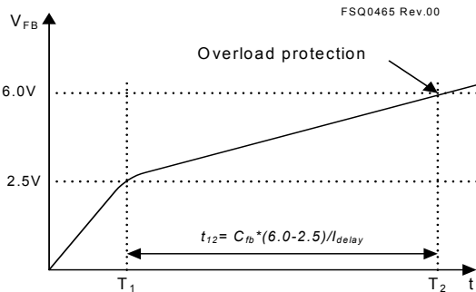
Figure 29. Overload Protection
