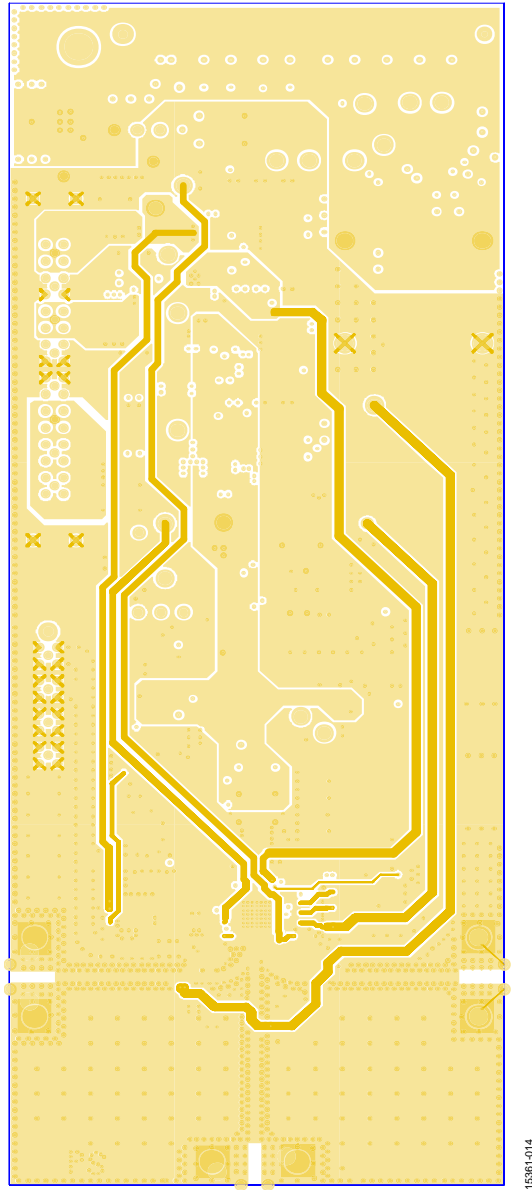
Figure 14. Evaluation Board Layer 3—Power
