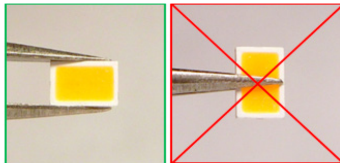
Figure 2. Correct handling (left) and incorrect handling (right) of LUXEON emitters.
