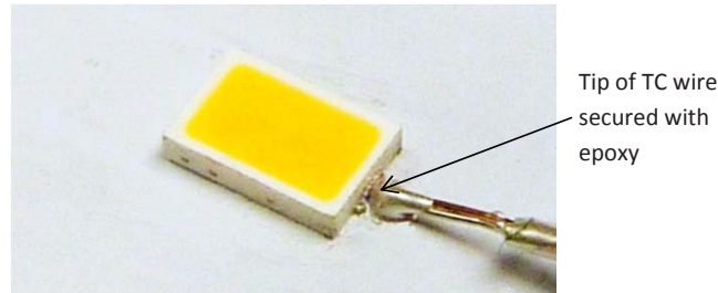
Figure 5. Photo showing actual placement of TC wire secured with thermal conductive epoxy. The thermal epoxy volume should be kept to minimum as shown.
