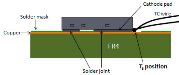
Figure 4. The recommended temperature measurement point T_s is located on the cathode copper layer of the PCB, closest to the package, partially touching the cathode pin. The picture above shows where to place the welding tip of the TC wire prior to dispensing any thermal conductive epoxy to secure the TC wire.
