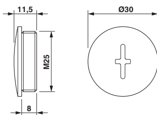
Dimensional drawing
