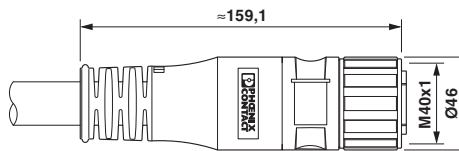
Dimensional drawing
