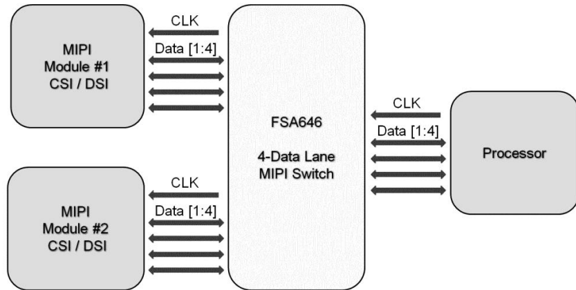
Figure 1. Typical Application
