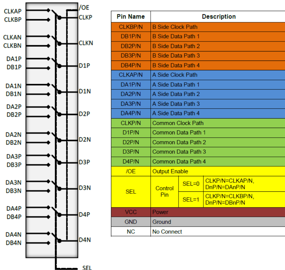
Figure 2. Analog Symbol
