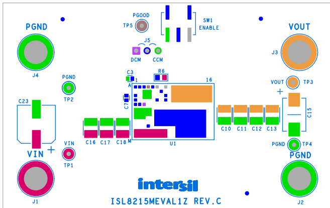
Figure 15. Silkscreen Top
