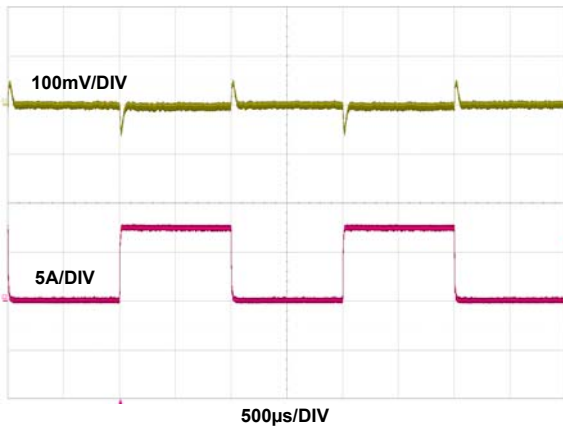
Figure 11. Transient Response, V_{OUT} = 3.3V , 0A to 7.5A, 2.5A/ \mu s Step Load, C_{OUT} = 4 \times 100\mu F Ceramic + 1x470 \mu F POSCAP
