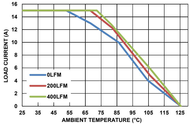
Figure 14. Derating Curve, V_{OUT} = 3.3V , C_{OUT} = 4 \times 100\mu F Ceramic + 1x470 \mu F POSCAP
