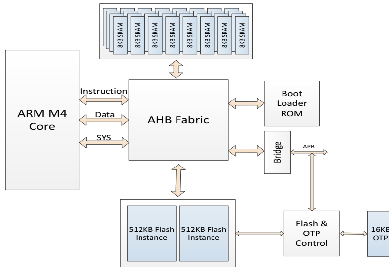
Figure 5. Block Diagram for Flash and OTP Memory Subsystem
