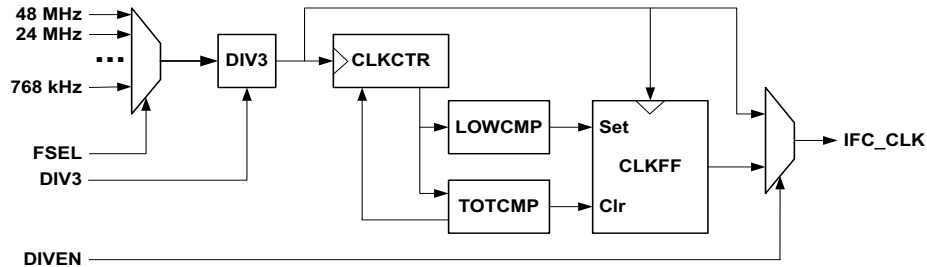
Figure 10. I 2 C/SPI Master Clock Generation
