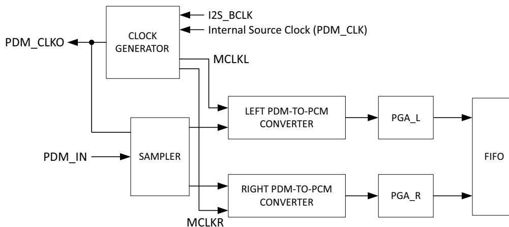
Figure 44. Stereo PDM to PCM Conversion Path
