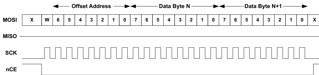
Figure 40. SPI Write Operation
