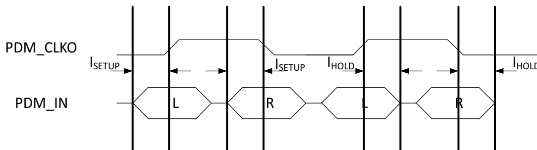
Figure 45. PDM Clock Timing Diagram
