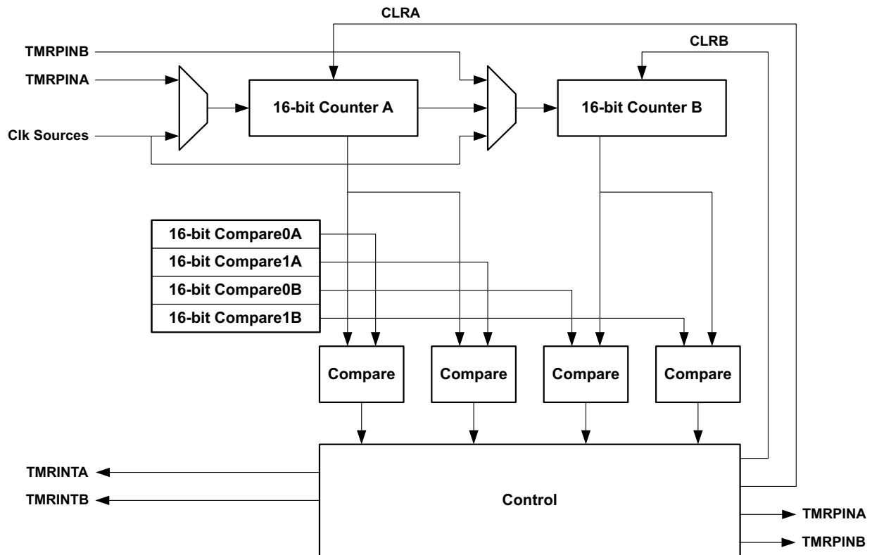
Figure 53. Block Diagram for One General Purpose Counter/Timer Pair
