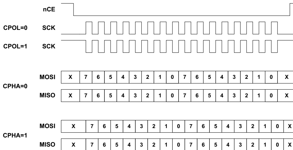
Figure 42. SPI CPOL and CPHA
