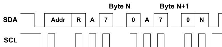
Figure 19. I 2 C Raw Read Operation
