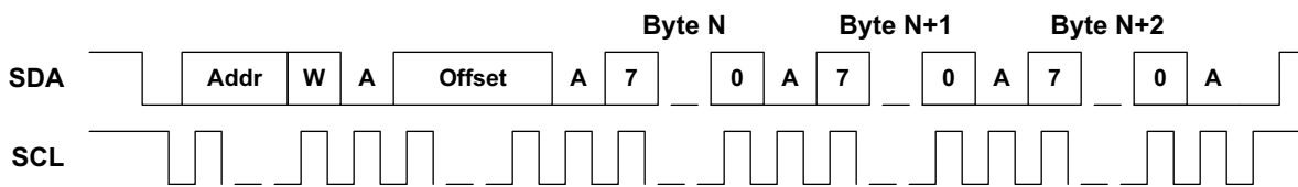
Figure 16. I 2 C Normal Write Operation
