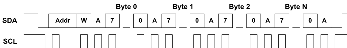
Figure 18. I 2 C Raw Write Operation
