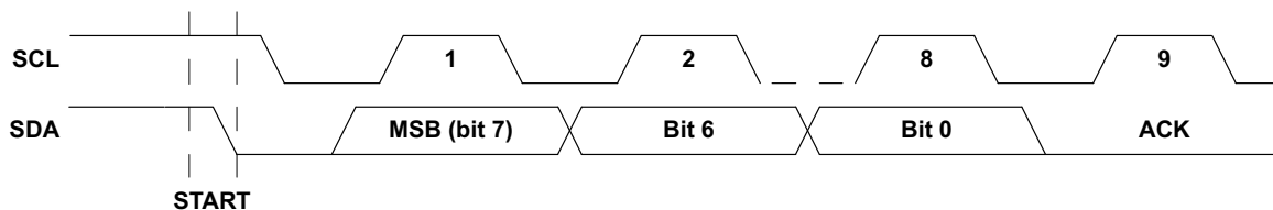
Figure 34. I 2 C Acknowledge
