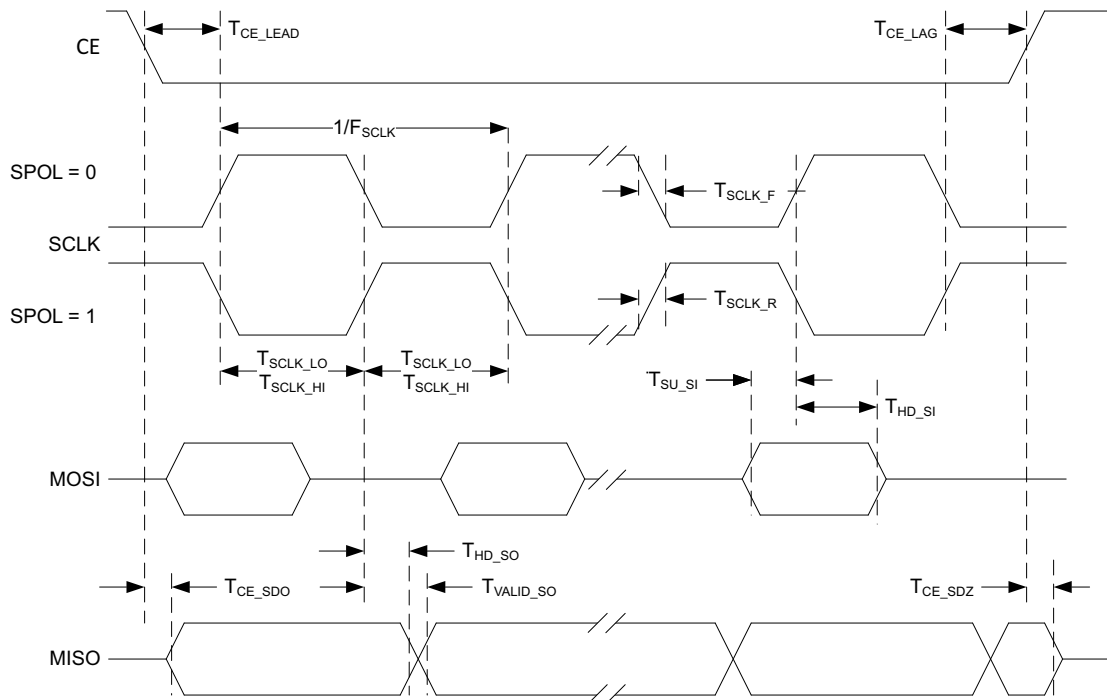
Figure 75. SPI Slave Mode, Phase = 0
