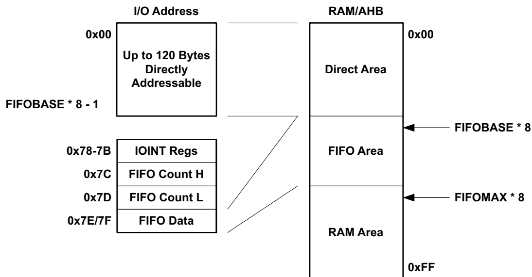
Figure 31. I 2 C/SPI Slave Module LRAM Addressing
