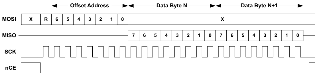
Figure 41. SPI Read Operation
