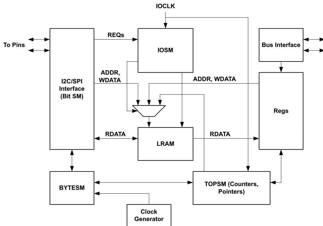
Figure 9. Block Diagram for the I 2 C/SPI Master Module
