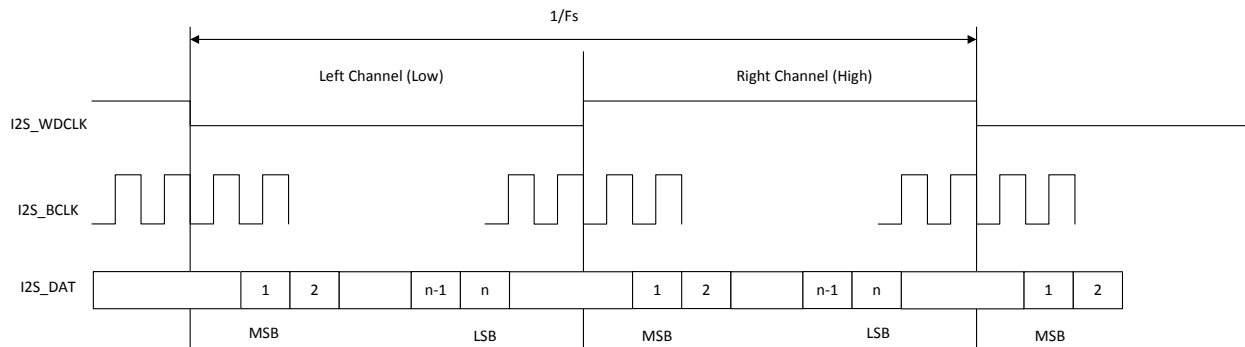
Figure 47. I 2 S Interface Data Format Timing
