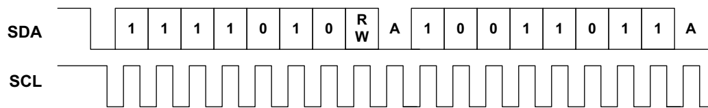
Figure 36. I 2 C 10-bit Address Operation
