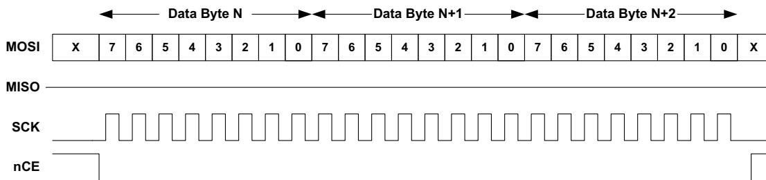
Figure 22. SPI Raw Write Operation
