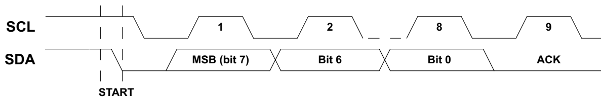
Figure 12. I 2 C Acknowledge
