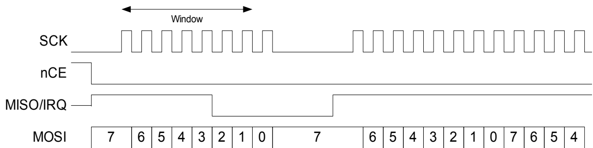
Figure 28. Flow Control in the Middle of a Write Transfer
