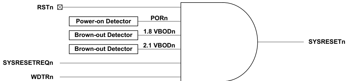
Figure 61. Block diagram for the Reset Generator Module
