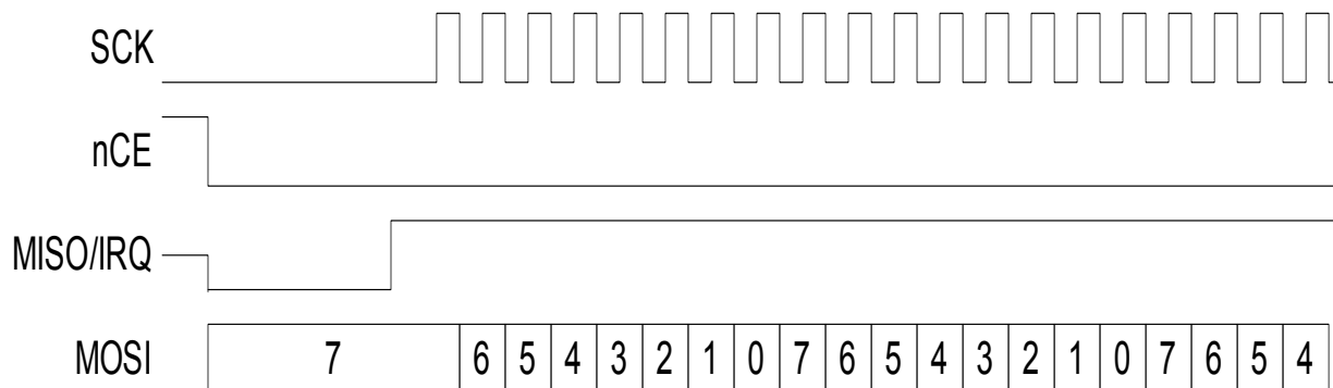
Figure 26. Flow Control at Beginning of a Write Transfer
