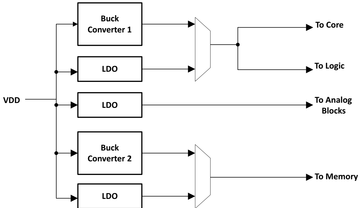
Figure 69. Block Diagram for the Voltage Regulator Module
