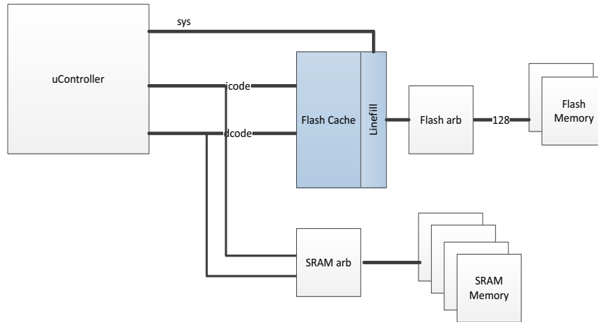
Figure 6. Block Diagram for Apollo2 with Flash Cache
