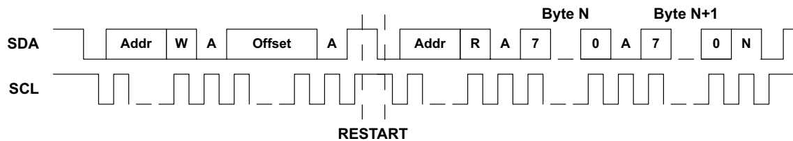
Figure 39. I 2 C Read Operation
