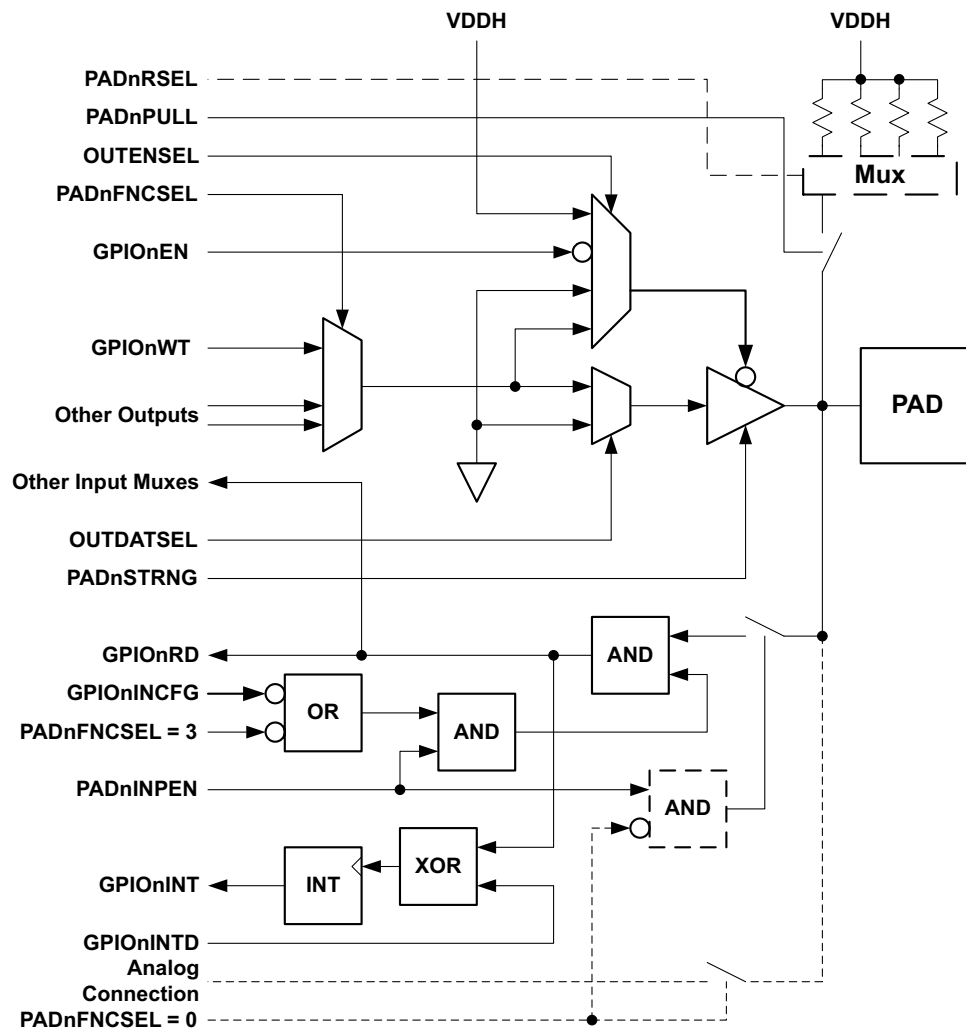
Figure 50. Pad Connection Details
