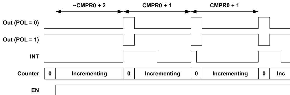
Figure 55. Counter/Timer Operation, FN = 1
