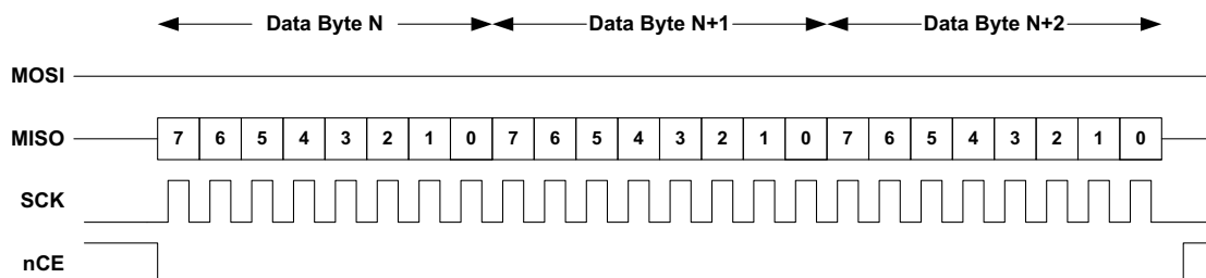
Figure 23. SPI Raw Read Operation
