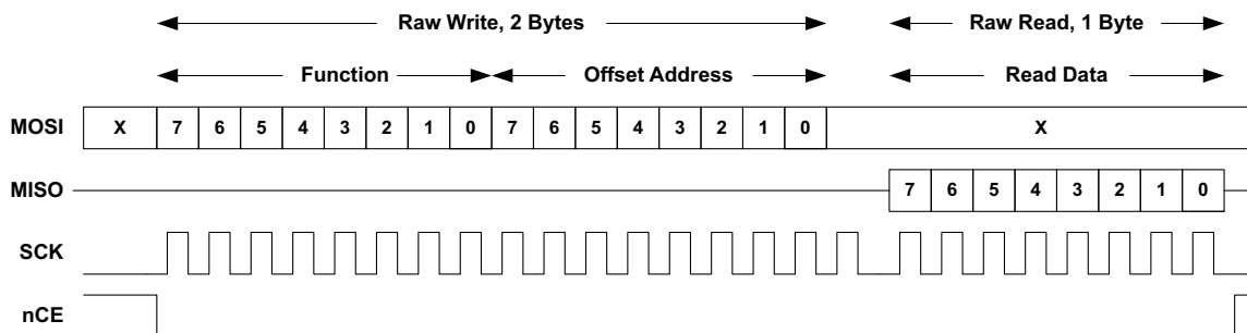
Figure 24. SPI Combined Operation
