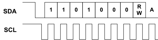
Figure 13. I 2 C 7-bit Address Operation
