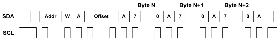
Figure 38. I 2 C Write Operation
