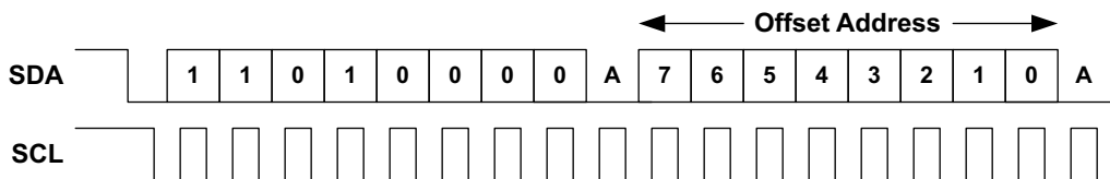
Figure 15. I 2 C Offset Address Transmission
