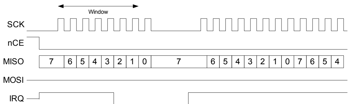
Figure 29. Flow Control in the Middle of a Read Transfer
