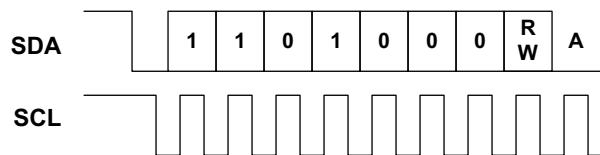
Figure 35. I 2 C 7-bit Address Operation
