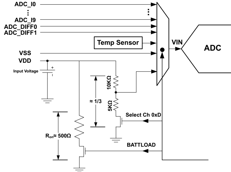
Figure 67. Switchable Battery Load
