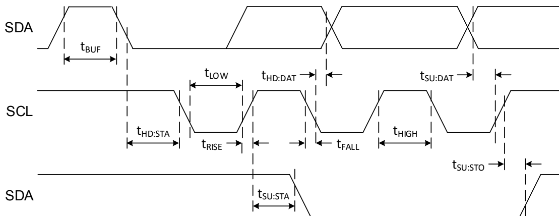
Figure 70. I 2 C Timing
