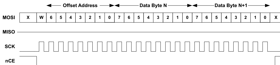
Figure 20. SPI Normal Write Operation
