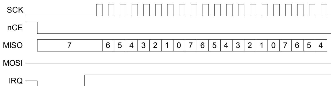
Figure 27. Flow Control at Beginning of a Raw Read Transfer
