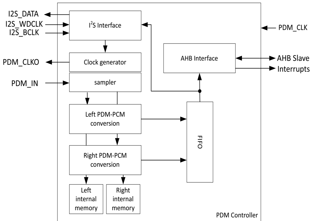
Figure 43. Block Diagram for PDM Module
