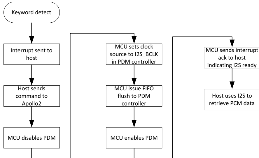
Figure 46. PDM Clock Source Switching Flow
