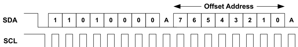
Figure 37. I 2 C Offset Address Transmission
