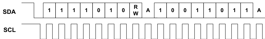
Figure 14. I 2 C 10-bit Address Operation
