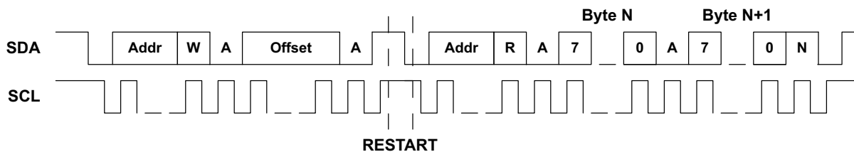
Figure 17. I 2 C Normal Read Operation
