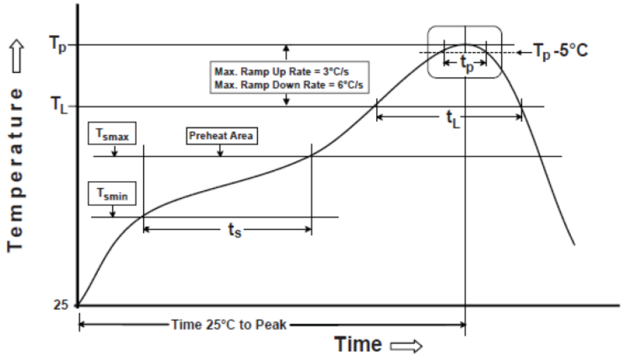
Figure 80. Reflow Soldering Diagram
