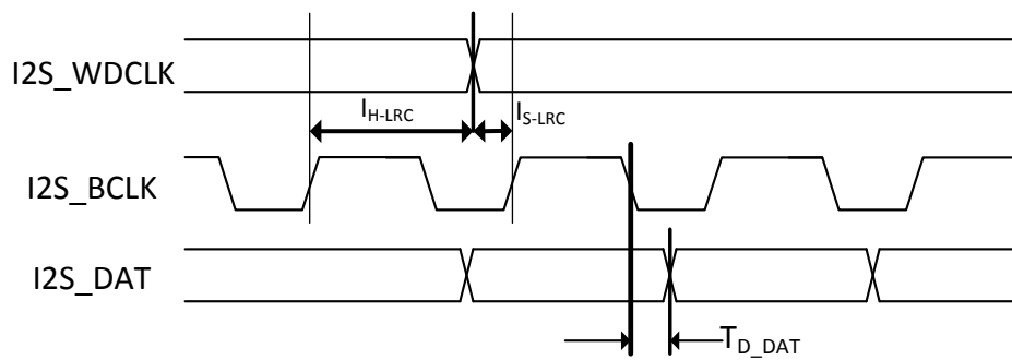
Figure 48. I 2 S Interface Setup and Hold Timing Diagram
