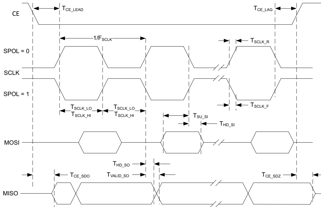
Figure 76. SPI Slave Mode, Phase = 1
