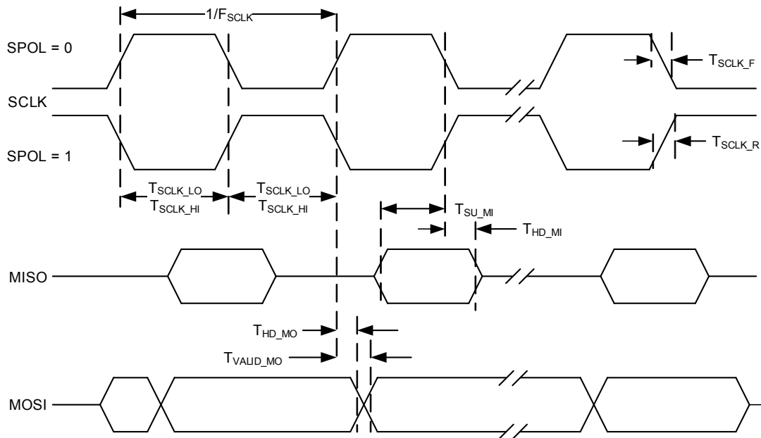
Figure 72. SPI Master Mode, Phase = 1
