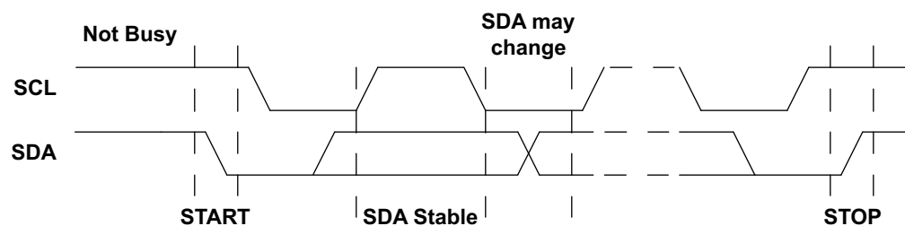
Figure 33. Basic I 2 C Conditions
