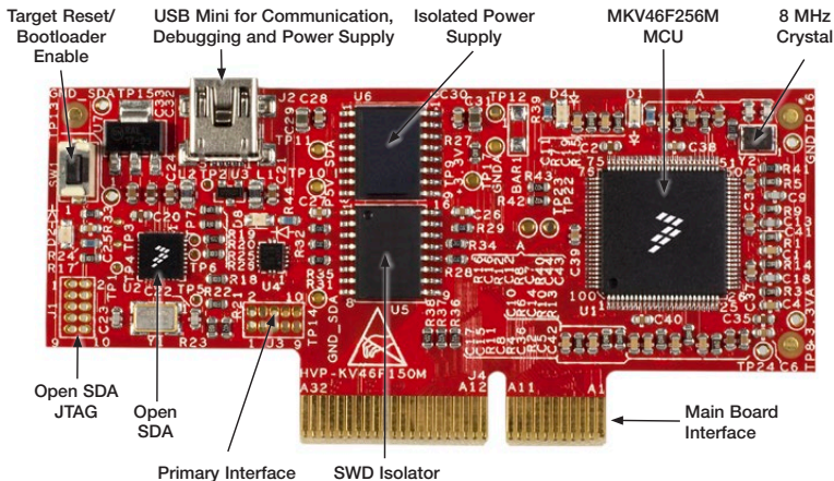
Figure 1: Front side of HVP-KV46F150M
