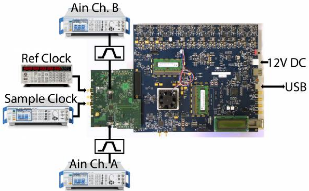
Figure 2. Evaluation Board Connection— AD9680-1000EBZ (on Left) and ADS7-V1EBZ (on Right)
