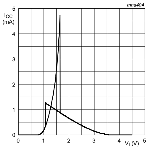
Fig 12. Typical 74AHCT1G17-Q100 transfer characteristics; V_{CC} = 4.5\text{ V}
