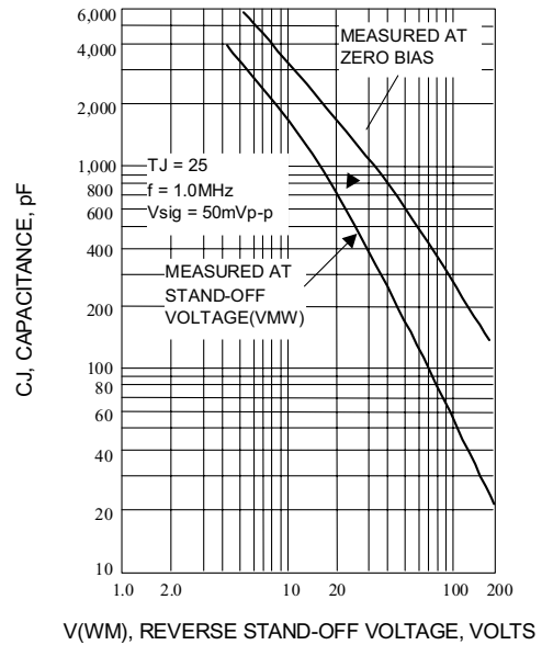
Fig. 4-TYPICAL JUNCTION CAPACITANCE
