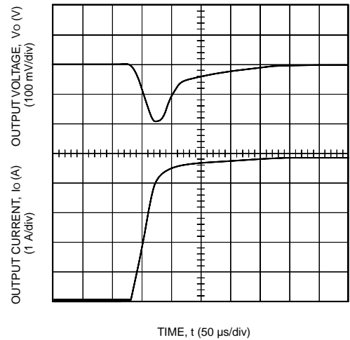
Figure 11. Typical JC100F Transient Response to Step Increase in Load from 50% to 75% of Full Load at Room Temperature and 28 V Input (Waveform Averaged to Eliminate Ripple Component.)
