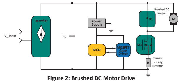
Figure 2: Brushed DC Motor Drive
