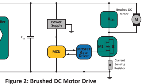
Figure 2: Brushed DC Motor Drive
