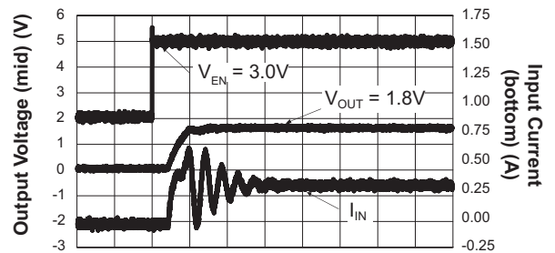
Startup Waveform
