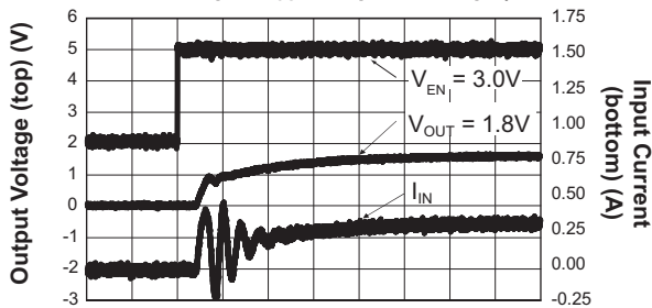
Startup Waveform
