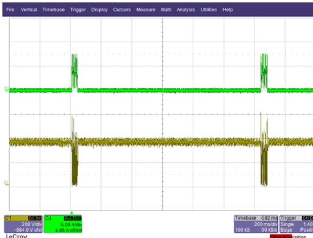
Figure 26 – 265 VAC, Full Load. Upper: I_{OUTPUT} , 5 A / div. Lower: V_{OUTPUT} , 200 V, 200 ms / div.
