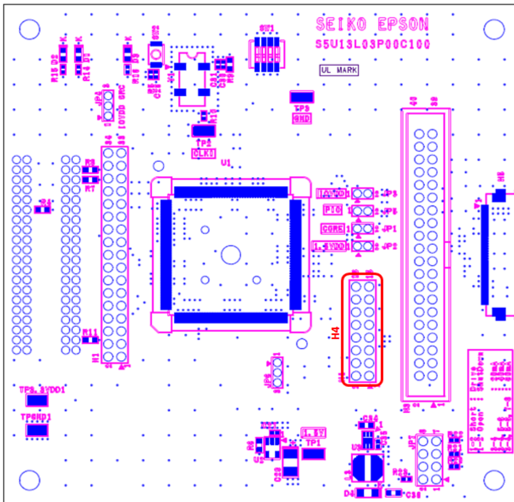
Figure 4-4: GPIO Connector Location (H4)
