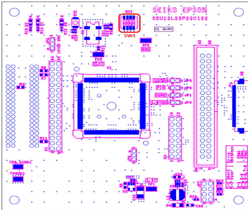
Figure 3-1: Configuration DIP Switch (SW1) Location
