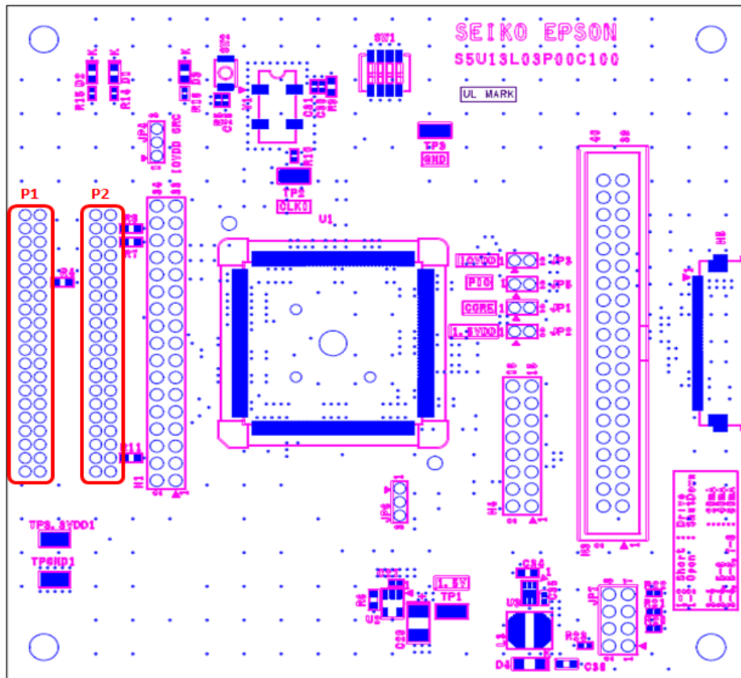
Figure 4-2: USB Adapter Connector Locations (P1 and P2)
