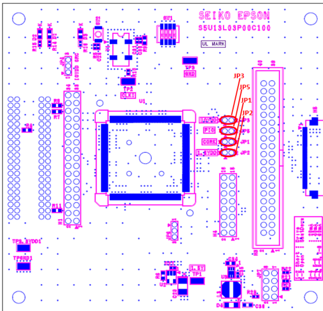
Figure 3-2: Configuration Jumper Locations (JP1, JP2, JP3, JP5)
