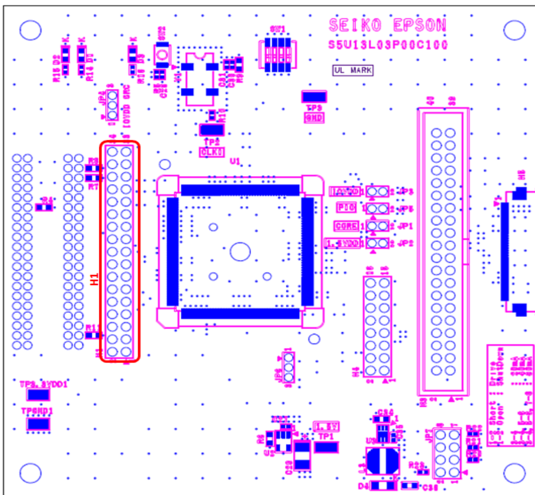
Figure 4-1: Host Bus Connector Location (H1)
