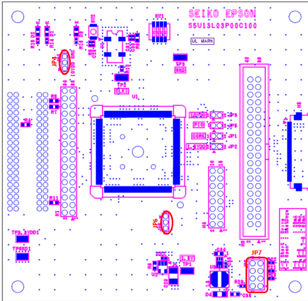
Figure 3-3: Configuration Jumper Location (JP4, JP6, JP7)
