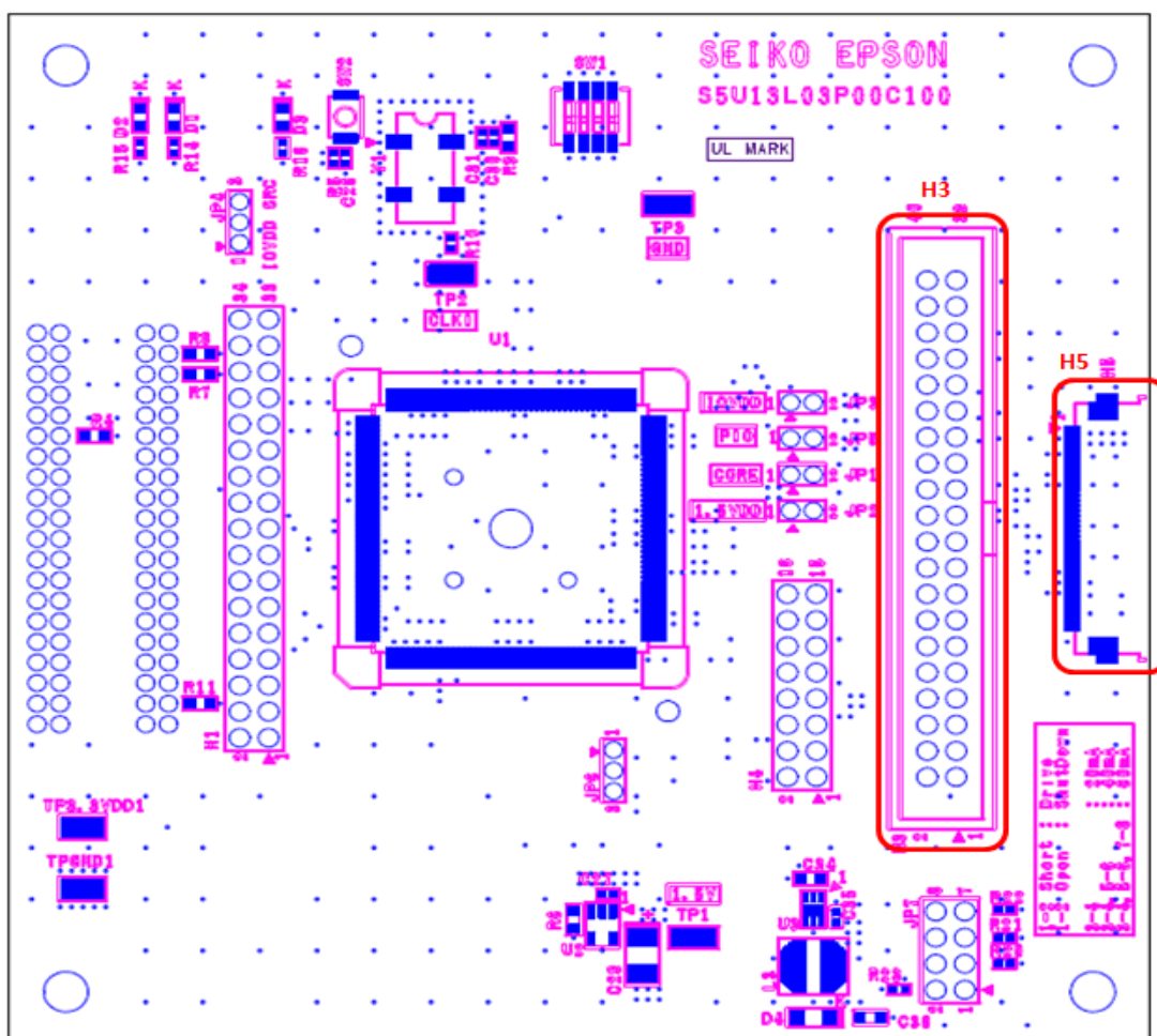
Figure 4-3: LCD Panel Connectors Location (H3, H5)
