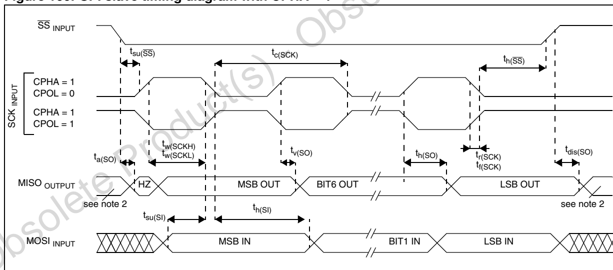
Figure 100. SPI slave timing diagram with CPHA = 1
