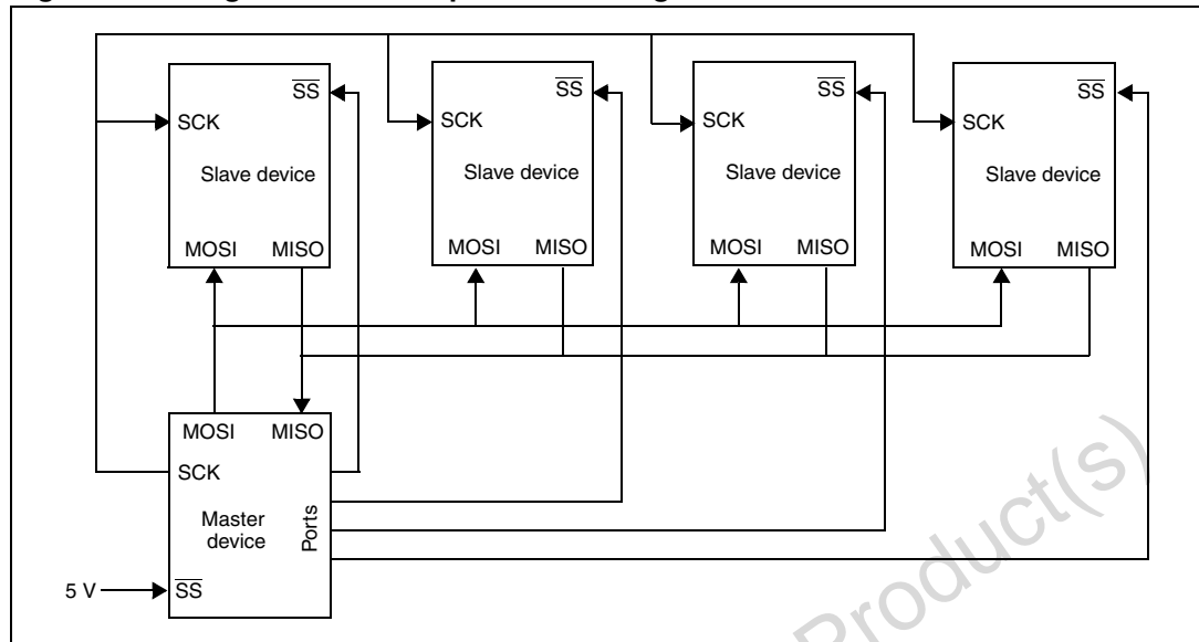
Figure 55. Single master/multiple slave configuration
