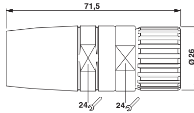
Dimensioned drawing
