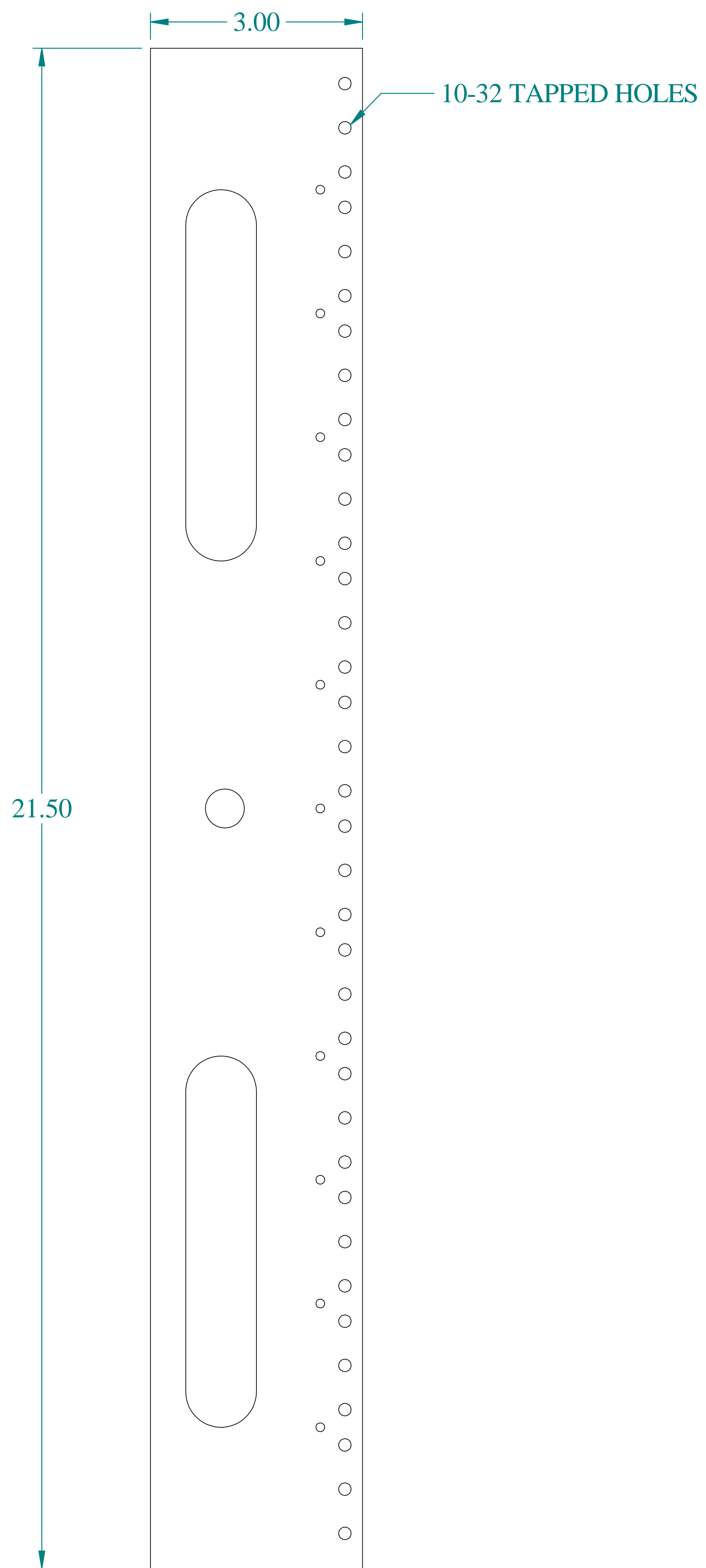
FRONT VIEW
