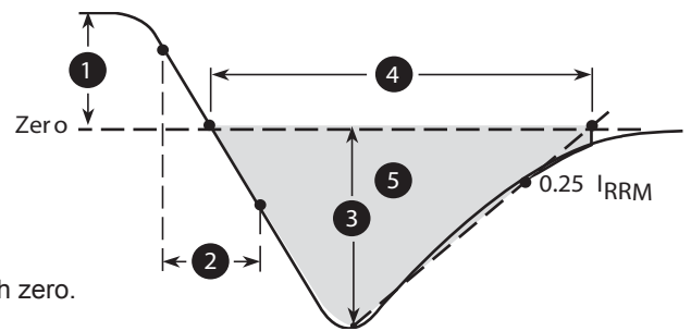
Figure 32. Diode Reverse Recovery Waveform Definition
