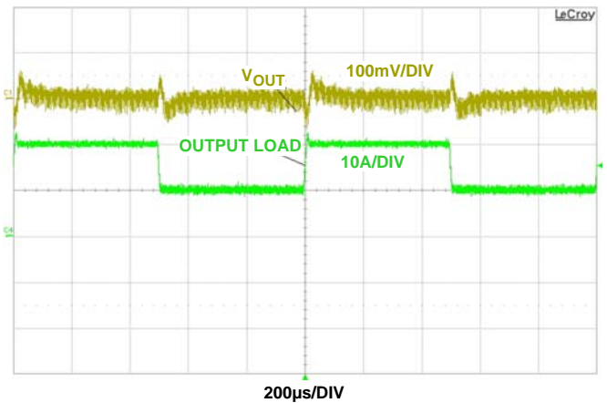
FIGURE 12. 10A -20A; 2A/ \mu s AT CCM MODE
