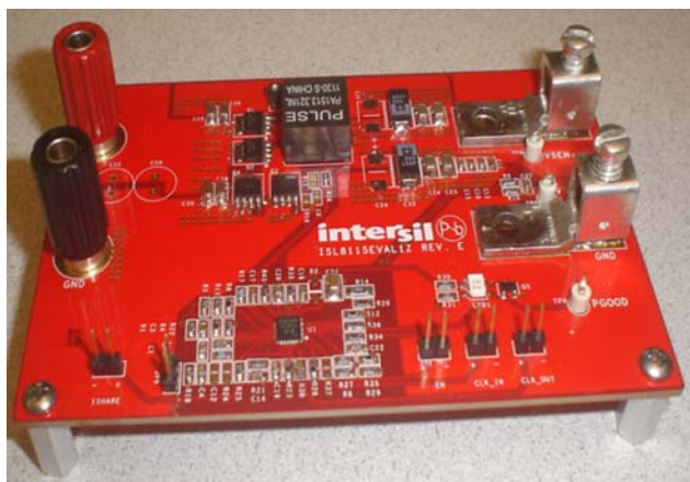
FIGURE 1. ISL8115EVAL1Z EVALUATION BOARD
