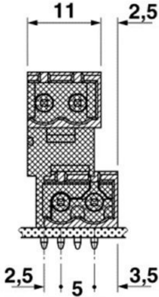
Dimensioned drawing
