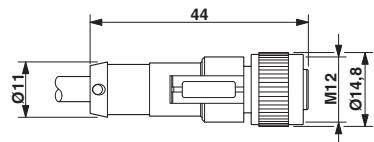
Dimensional drawing
