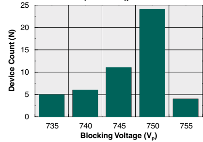
Typical Blocking Voltage Distribution ( I_F=0\text{mA} , T_A=25^\circ\text{C} )
