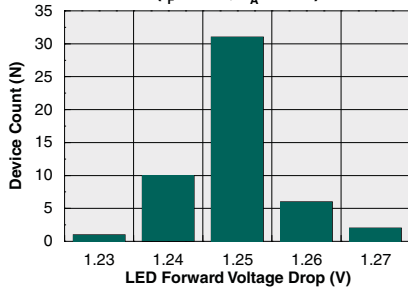
Typical LED Forward Voltage Drop ( I_F=5\text{mA} , T_A=25^\circ\text{C} )
