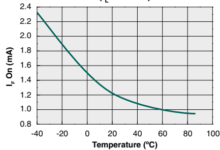
Typical I_F for Switch Operation vs. Temperature ( I_L=250\text{mA} )
