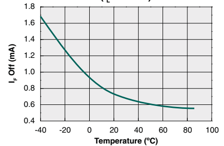
Typical I_F for Switch Dropout vs. Temperature ( I_L=250\text{mA} )
