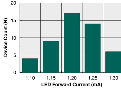
Typical I_F for Switch Operation ( I_L=250\text{mA} , T_A=25^\circ\text{C} )
