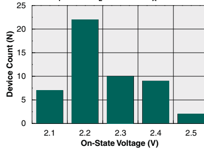
Typical On-State Output Forward Voltage Distribution ( I_F=5\text{mA} , I_L=250\text{mA} , T_A=25^\circ\text{C} )
