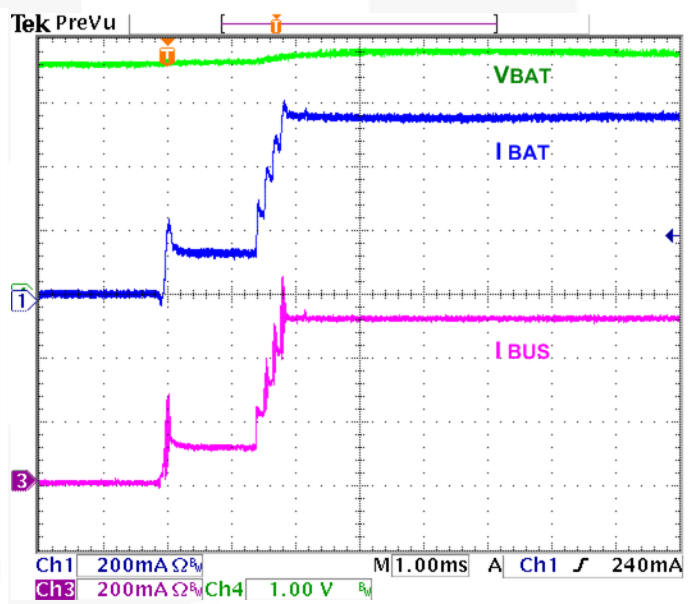
Figure 15. Charger Startup with HZ_MODE Bit Reset, I_{\text{NLIM}}=500\text{ mA} , I_{\text{CHARGE}}=950\text{ mA} , V_{\text{REG}}=4.2\text{ V} , V_{\text{BAT}}=3.6\text{ V}
