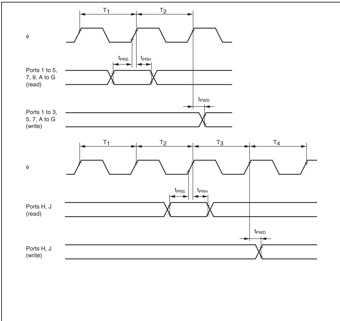
Figure 24.14 I/O Port Input/Output Timing
