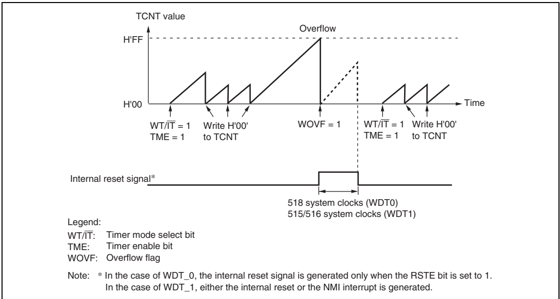
Figure 12.2 Watchdog Timer Mode Operation
