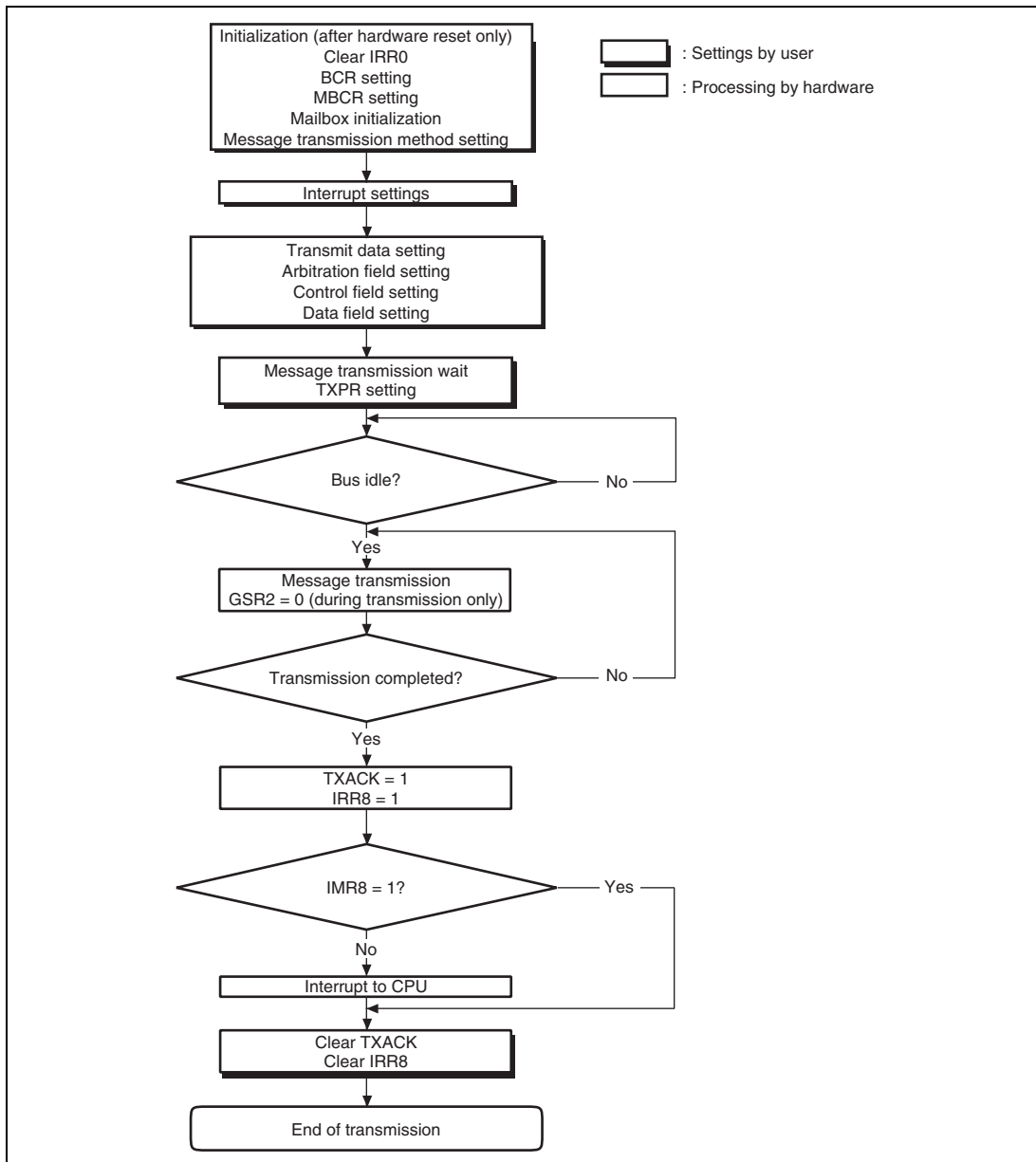
Figure 18.9 Transmission Flowchart
