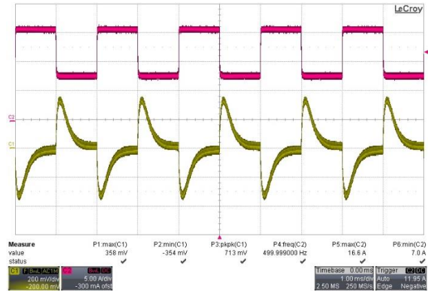
Figure 14: Load transient V_o (1.0ms/div), 8.5A <-> 17A, 2A/µs CH1: V_o (200 mV/div) CH2: I_o (5 A/div)
