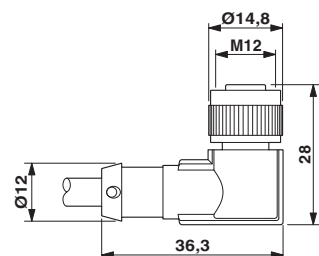
Socket M12 x 1, angled, with LED
