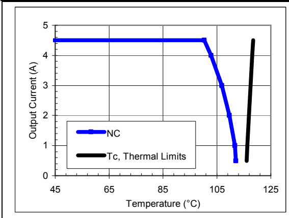
Vo=0.7V, Vin=12V maximum output current vs. ambient temperature at nominal input voltage for natural convection (60lfm) with airflow from pin 7 to pin 3.
