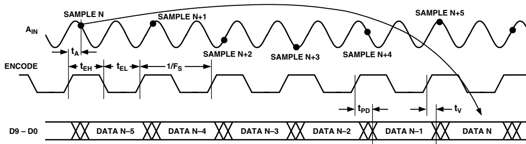
Figure 1. Timing Diagram
