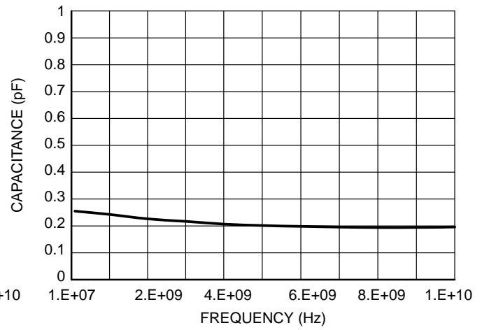
Figure 4. Typical Capacitance over Frequency ESD7461N2T5G (SOD882)
